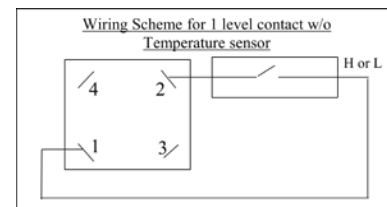
1 Level Contact w/o Temp Switch
