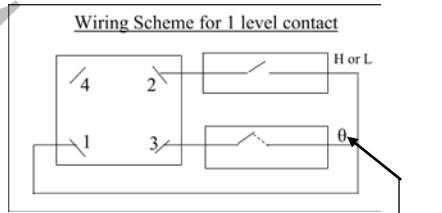
1 Level Contact
